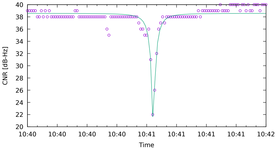
CNR fit for G06 on HuaweiP40 - drive 1 (DOY263)
