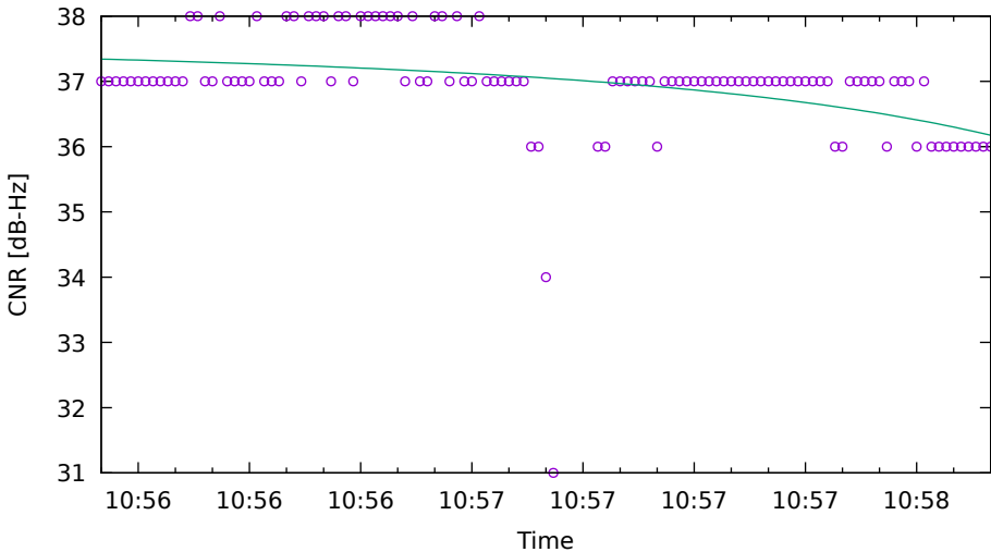
CNR fit for G06 on HuaweiP40 - drive 10 (DOY263)
