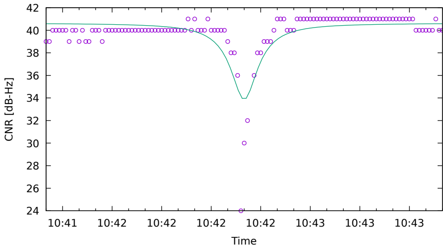
CNR fit for G06 on HuaweiP40 - drive 2 (DOY263)
