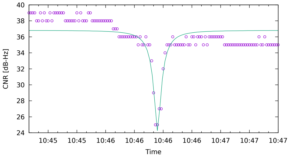
CNR fit for G06 on HuaweiP40 - drive 4 (DOY263)
