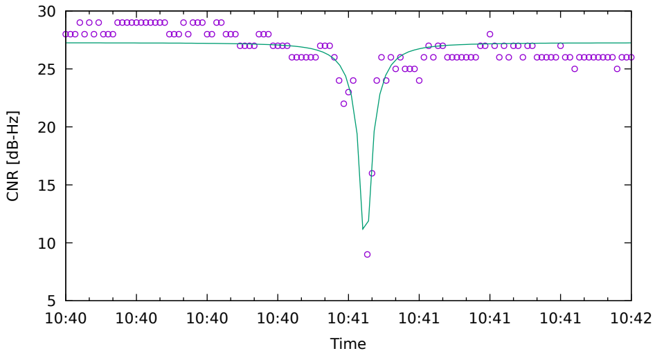
CNR fit for G09 on HuaweiP40 - drive 1 (DOY263)
