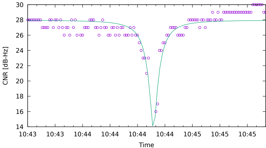
CNR fit for G09 on HuaweiP40 - drive 3 (DOY263)
