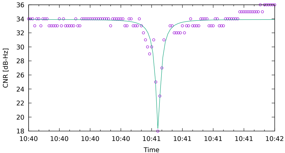
CNR fit for G17 on HuaweiP40 - drive 1 (DOY263)
