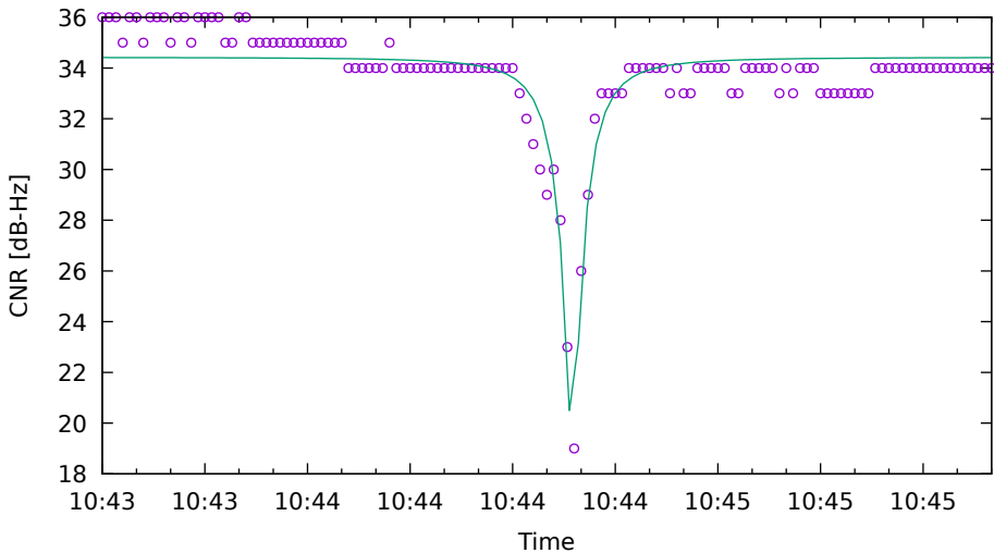
CNR fit for G17 on HuaweiP40 - drive 3 (DOY263)
