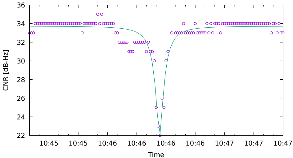
CNR fit for G17 on HuaweiP40 - drive 4 (DOY263)
