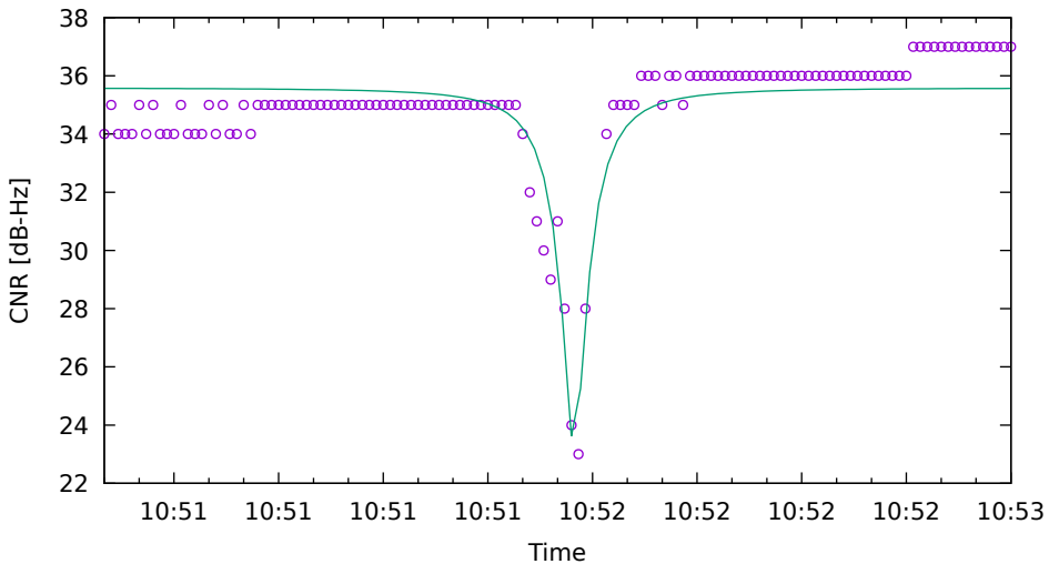
CNR fit for G17 on HuaweiP40 - drive 7 (DOY263)
