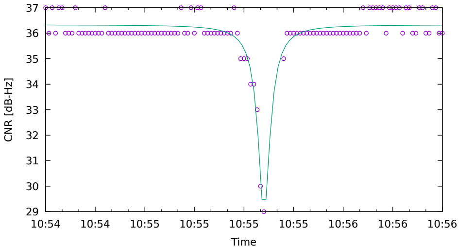
CNR fit for G17 on HuaweiP40 - drive 9 (DOY263)
