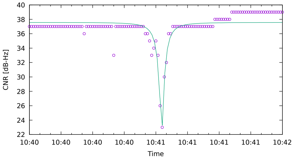
CNR fit for G19 on HuaweiP40 - drive 1 (DOY263)
