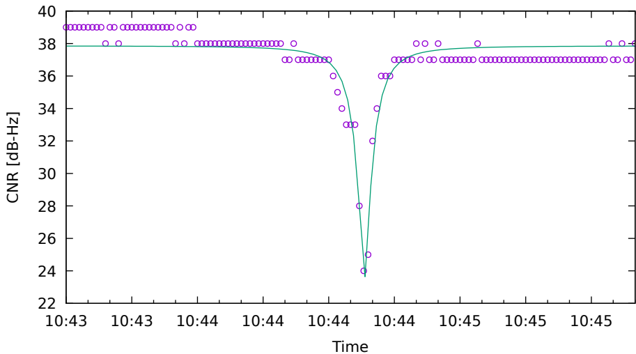
CNR fit for G19 on HuaweiP40 - drive 3 (DOY263)
