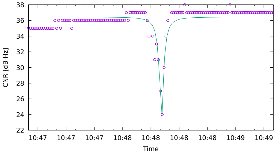
CNR fit for G19 on HuaweiP40 - drive 5 (DOY263)
