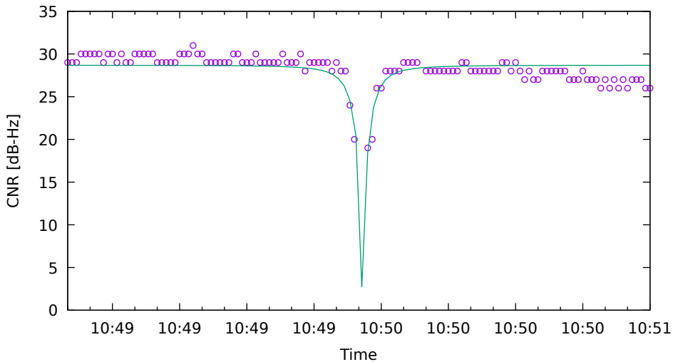
CNR fit for G22 on HuaweiP40 - drive 6 (DOY263)
