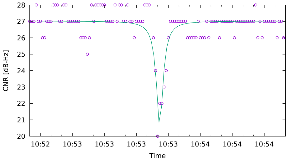
CNR fit for G22 on HuaweiP40 - drive 8 (DOY263)
