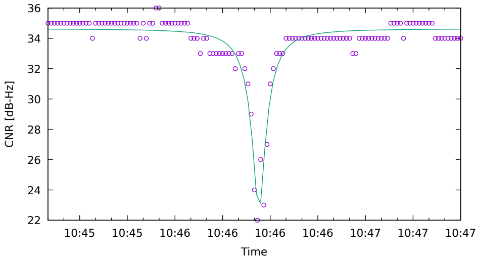
CNR fit for G31 on HuaweiP40 - drive 4 (DOY263)
