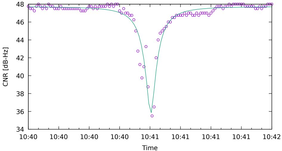
CNR fit for C11 on SamsungS20 - drive 1 (DOY263)
