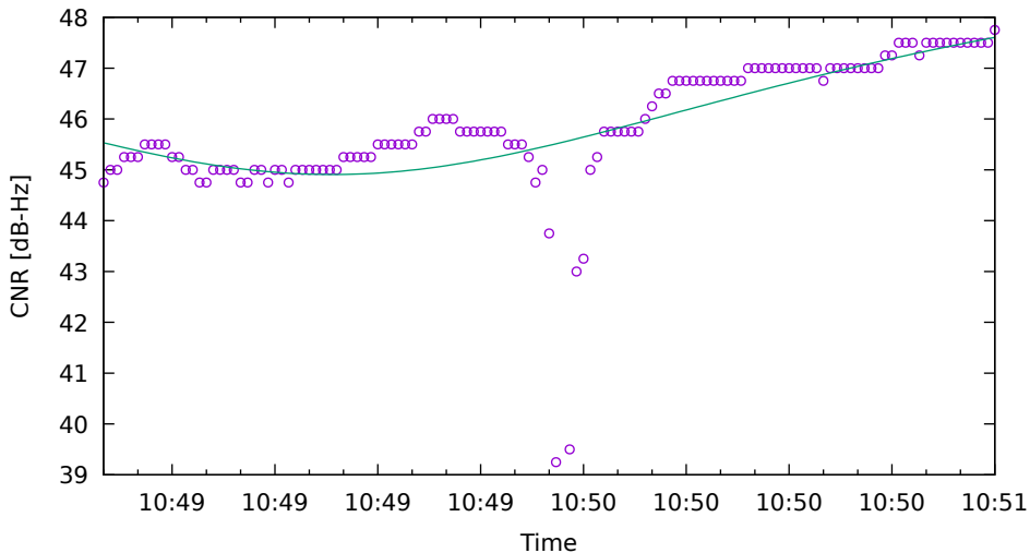
CNR fit for C11 on SamsungS20 - drive 6 (DOY263)
