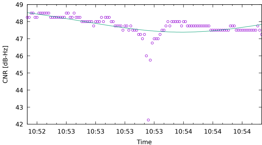
CNR fit for C11 on SamsungS20 - drive 8 (DOY263)
