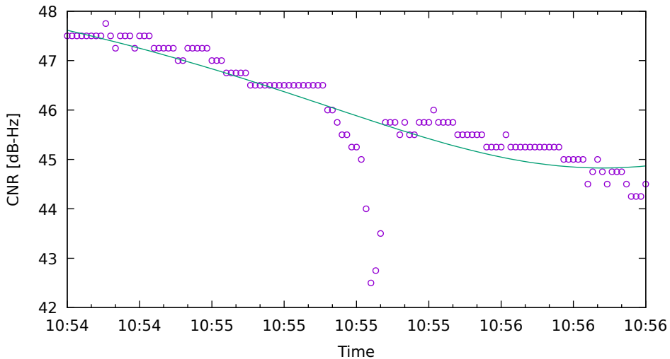
CNR fit for C11 on SamsungS20 - drive 9 (DOY263)
