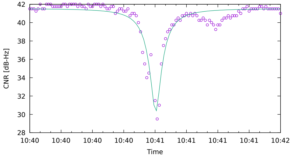
CNR fit for C16 on SamsungS20 - drive 1 (DOY263)
