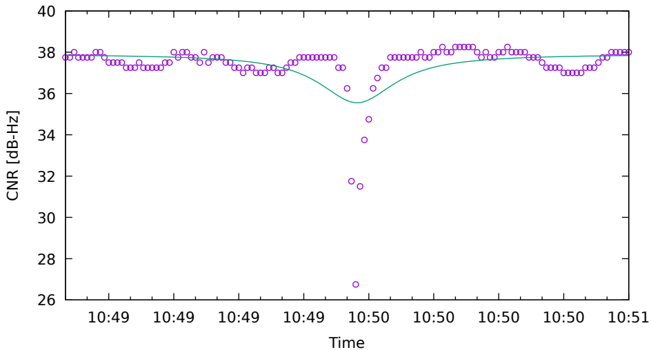
CNR fit for C16 on SamsungS20 - drive 6 (DOY263)
