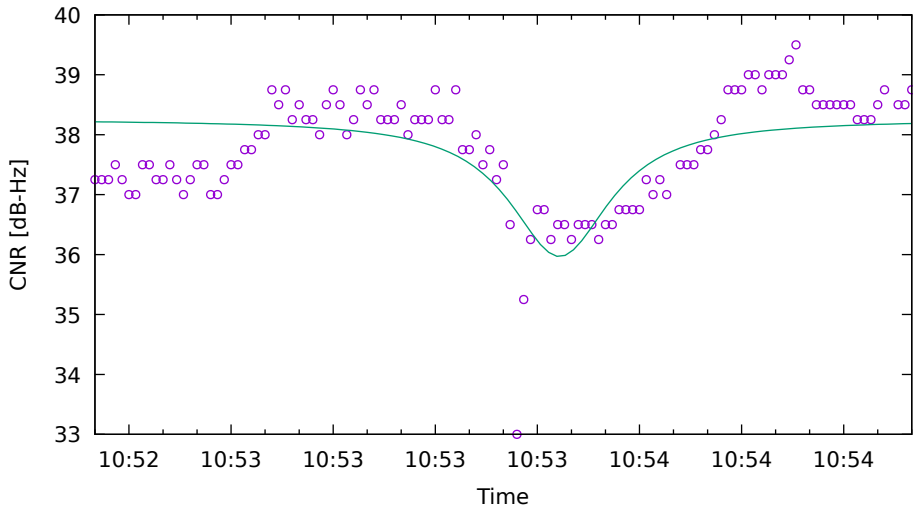
CNR fit for C16 on SamsungS20 - drive 8 (DOY263)
