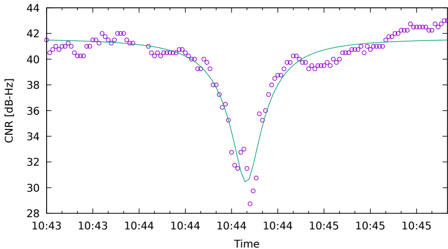
CNR fit for C28 on SamsungS20 - drive 3 (DOY263)
