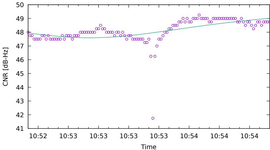
CNR fit for C28 on SamsungS20 - drive 8 (DOY263)
