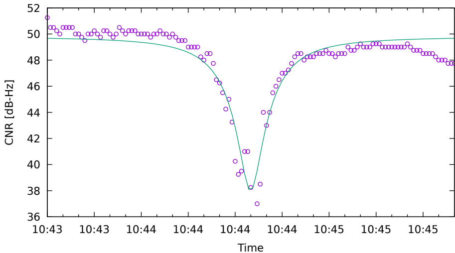
CNR fit for C33 on SamsungS20 - drive 3 (DOY263)
