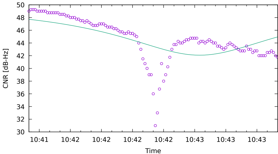
CNR fit for C34 on SamsungS20 - drive 2 (DOY263)
