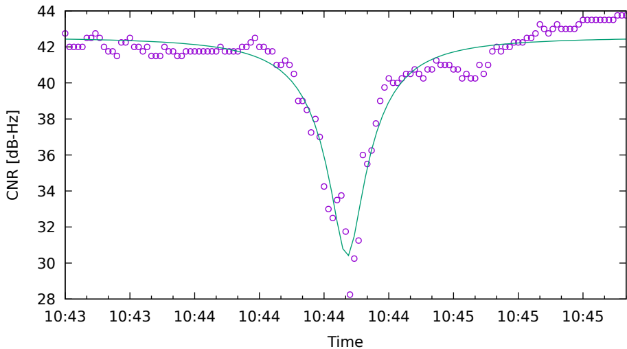
CNR fit for C34 on SamsungS20 - drive 3 (DOY263)
