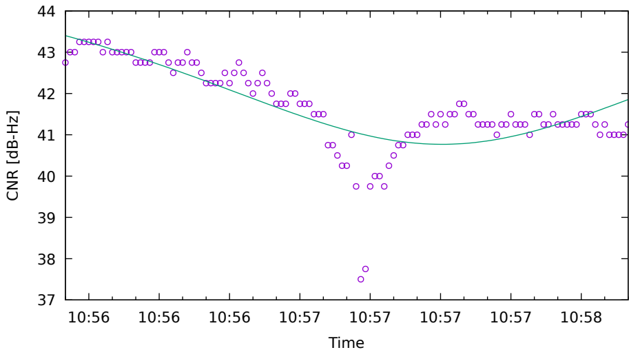
CNR fit for E04 on SamsungS20 - drive 10 (DOY263)
