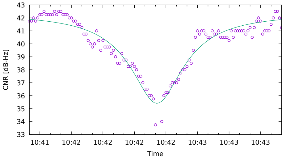
CNR fit for E11 on SamsungS20 - drive 2 (DOY263)
