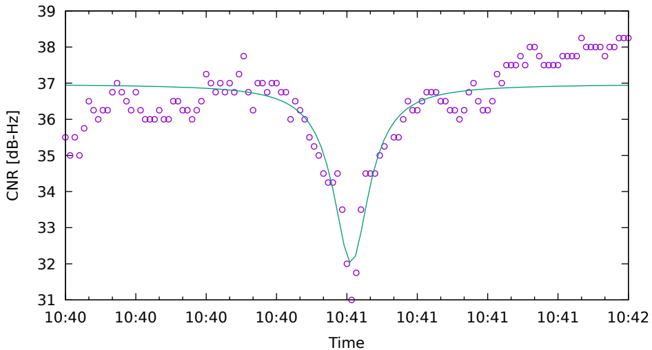
CNR fit for E19 on SamsungS20 - drive 1 (DOY263)
