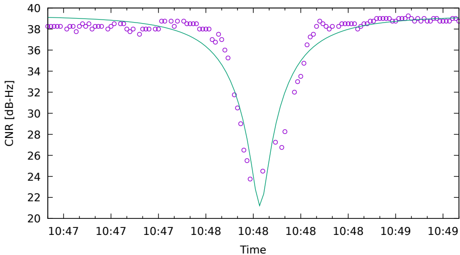
CNR fit for E19 on SamsungS20 - drive 5 (DOY263)
