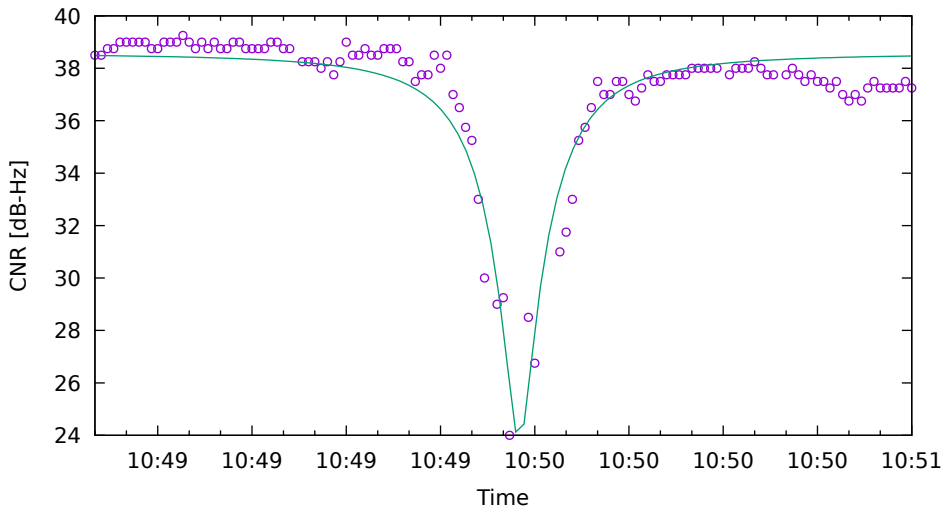
CNR fit for E19 on SamsungS20 - drive 6 (DOY263)
