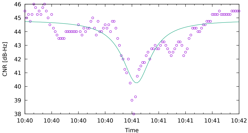
CNR fit for G01 on SamsungS20 - drive 1 (DOY263)
