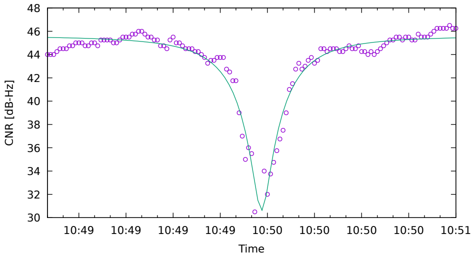
CNR fit for G01 on SamsungS20 - drive 6 (DOY263)
