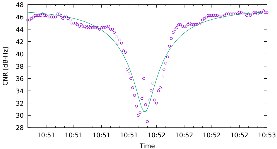
CNR fit for G01 on SamsungS20 - drive 7 (DOY263)
