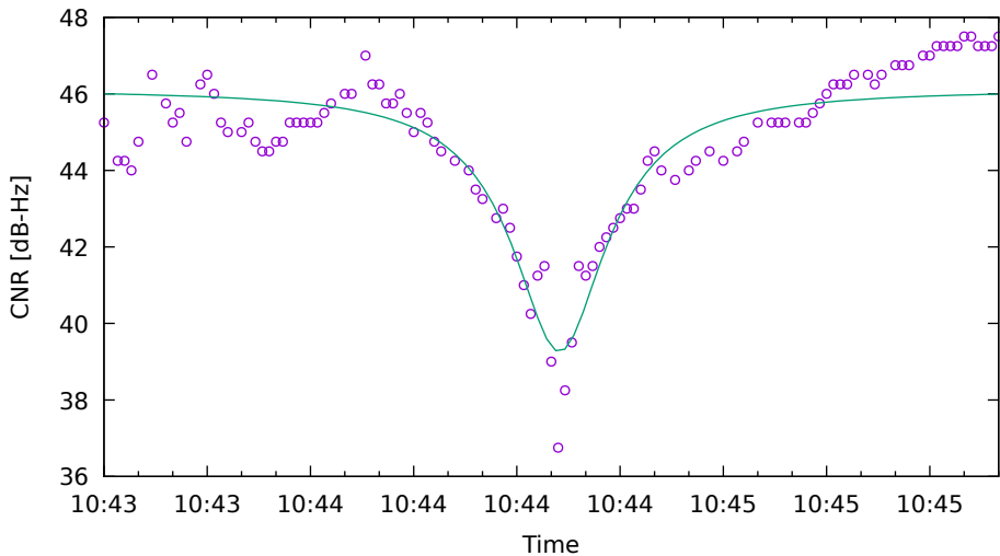
CNR fit for G03 on SamsungS20 - drive 3 (DOY263)
