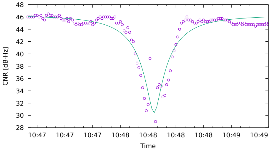
CNR fit for G03 on SamsungS20 - drive 5 (DOY263)
