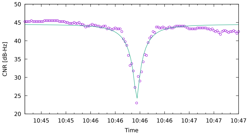
CNR fit for G04 on SamsungS20 - drive 4 (DOY263)
