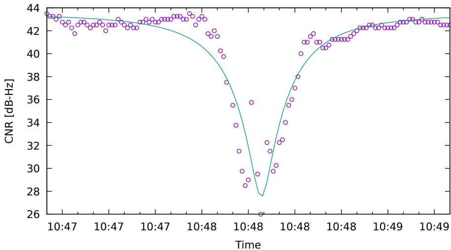
CNR fit for G04 on SamsungS20 - drive 5 (DOY263)
