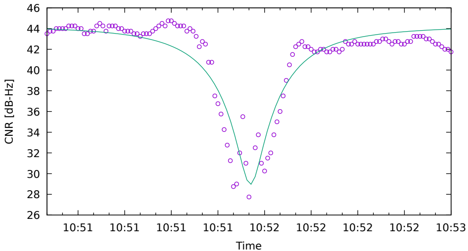
CNR fit for G04 on SamsungS20 - drive 7 (DOY263)
