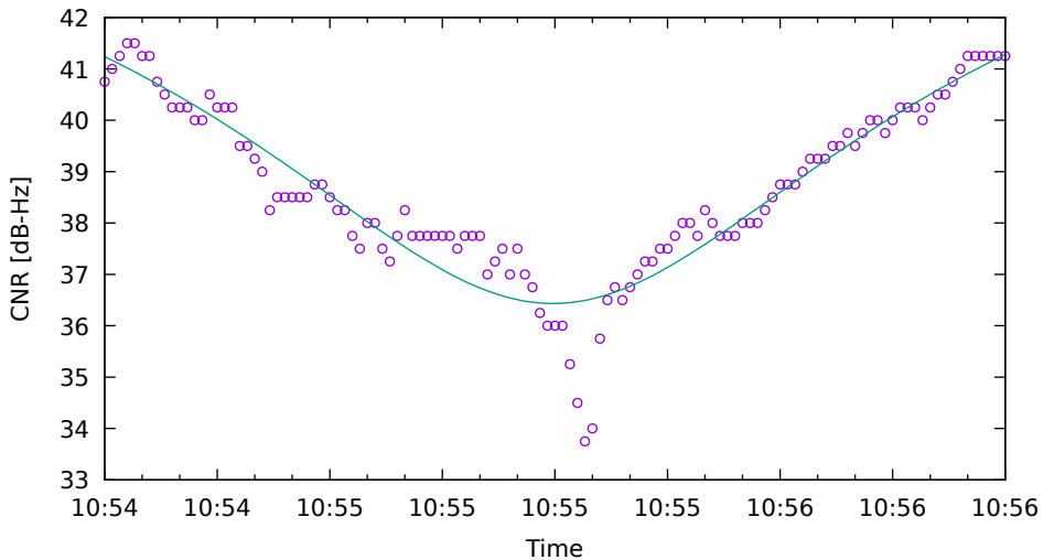
CNR fit for G04 on SamsungS20 - drive 9 (DOY263)
