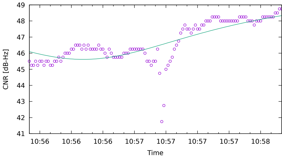
CNR fit for G06 on SamsungS20 - drive 10 (DOY263)
