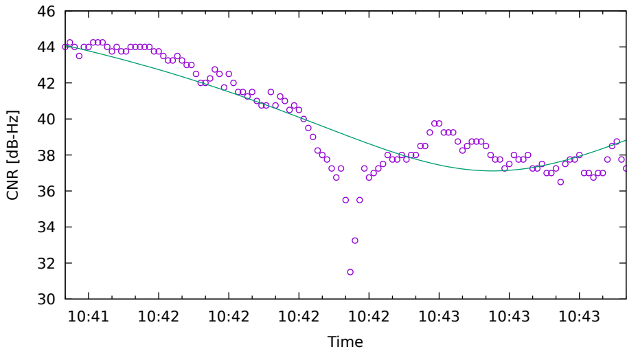
CNR fit for G06 on SamsungS20 - drive 2 (DOY263)
