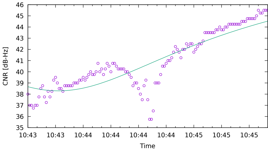
CNR fit for G06 on SamsungS20 - drive 3 (DOY263)
