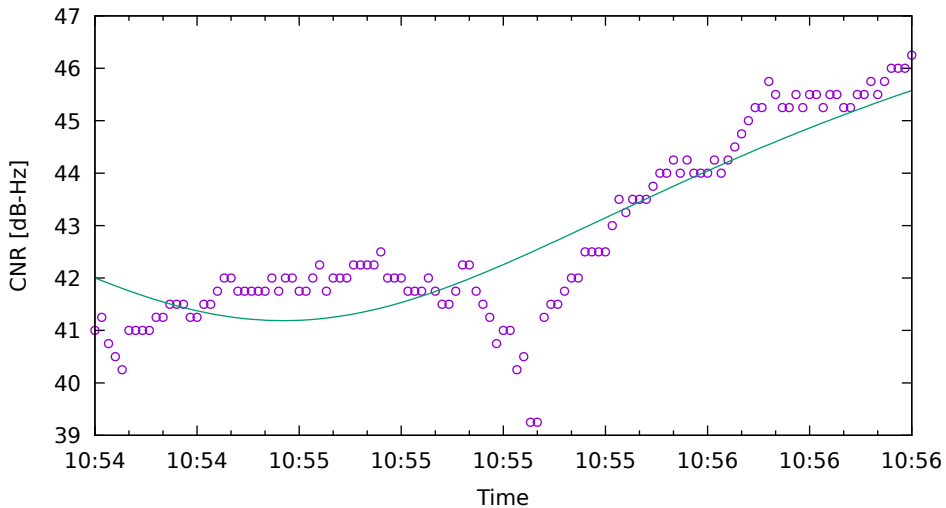
CNR fit for G06 on SamsungS20 - drive 9 (DOY263)
