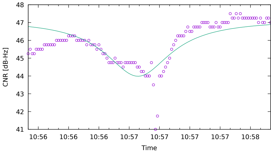
CNR fit for G09 on SamsungS20 - drive 10 (DOY263)
