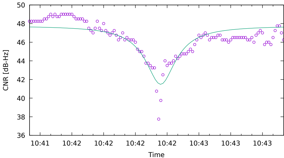
CNR fit for G09 on SamsungS20 - drive 2 (DOY263)
