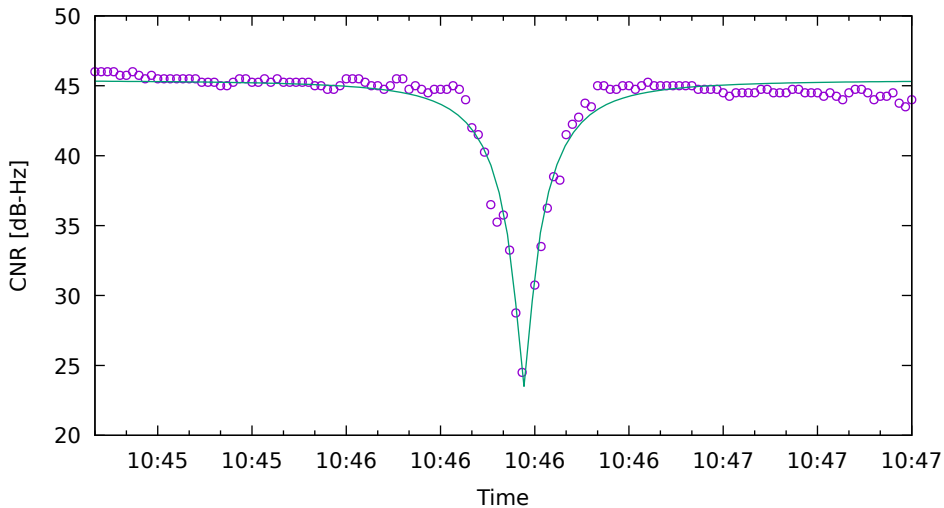
CNR fit for G09 on SamsungS20 - drive 4 (DOY263)
